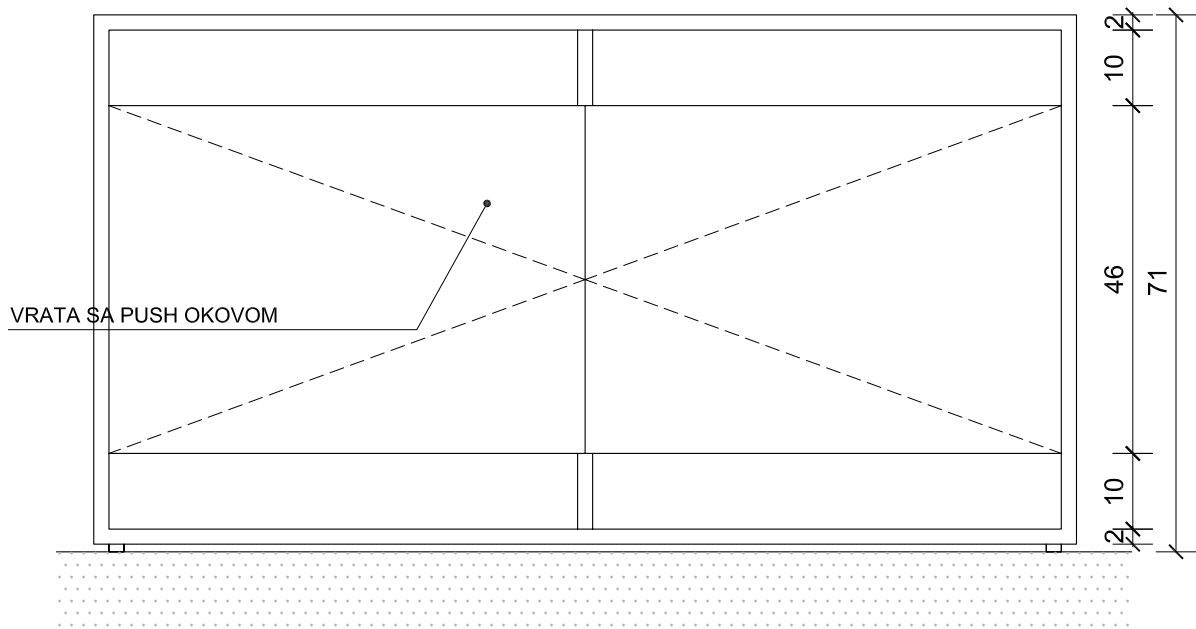
POGLED 2-2
