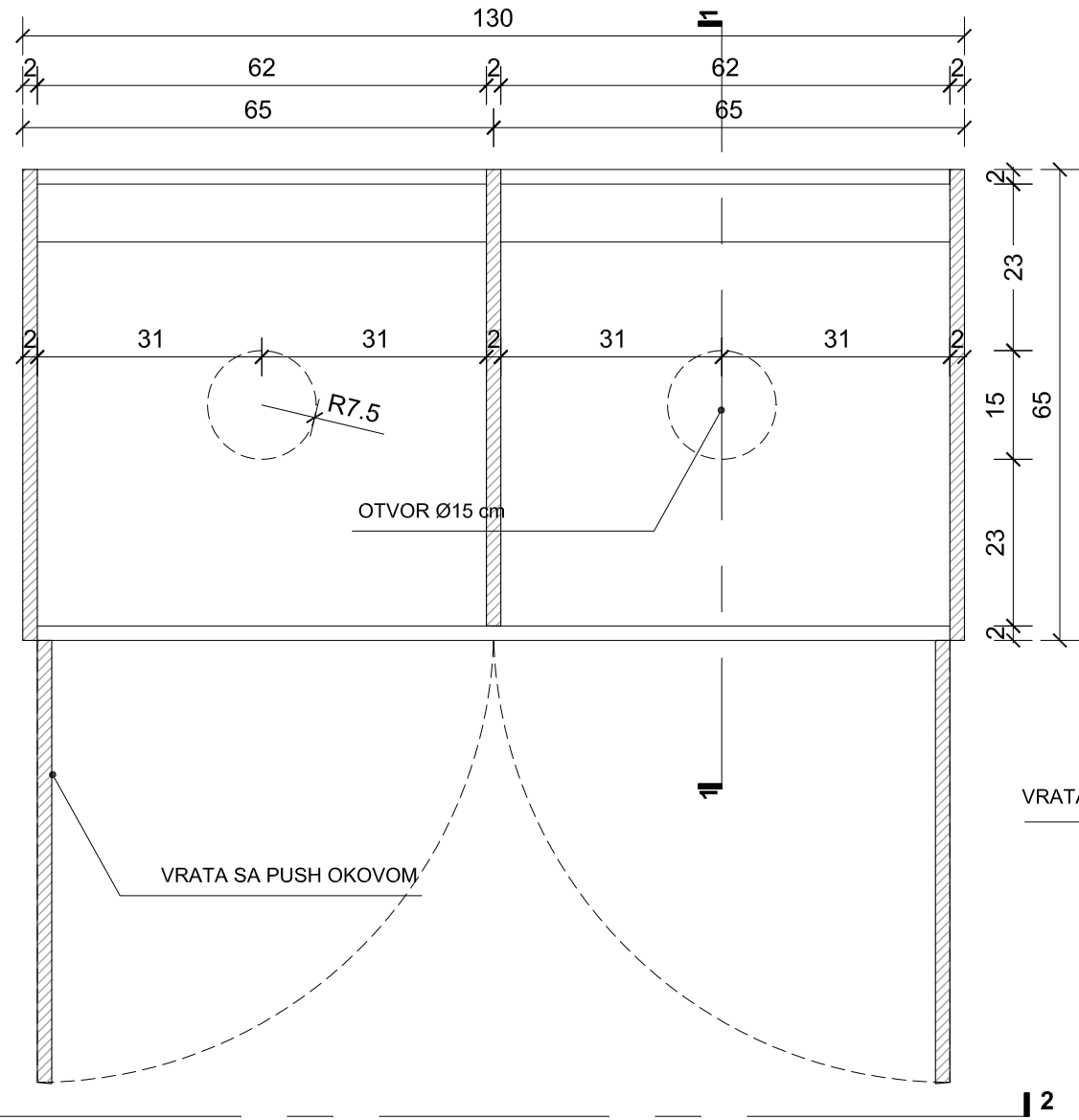
POGLED 2-2
